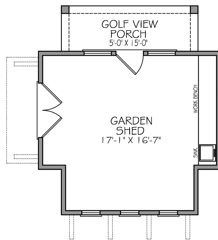
GARDEN SHED PLAN 8'-1 1/2" CEILING HEIGHT (B.N.O.) SCALE: 1/4" = 1'-0"
